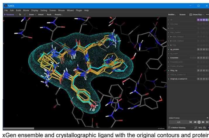
Figure 7.19 Final xGen ensemble.
