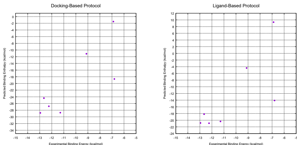
Figure 7.30 A comparison of results for the structure-based (left) and ligand-based (right) ranking protocols.
