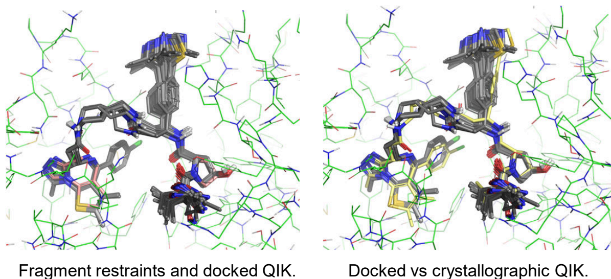
Figure 7.23 Docked QIK relative to the QIY warhead fragments and the crystallographic QIK ligand.
