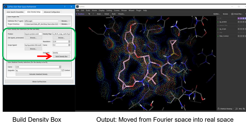
Figure 7.3 Step 1 of xGen ensemble generation: Move from Fourier space into real space.
