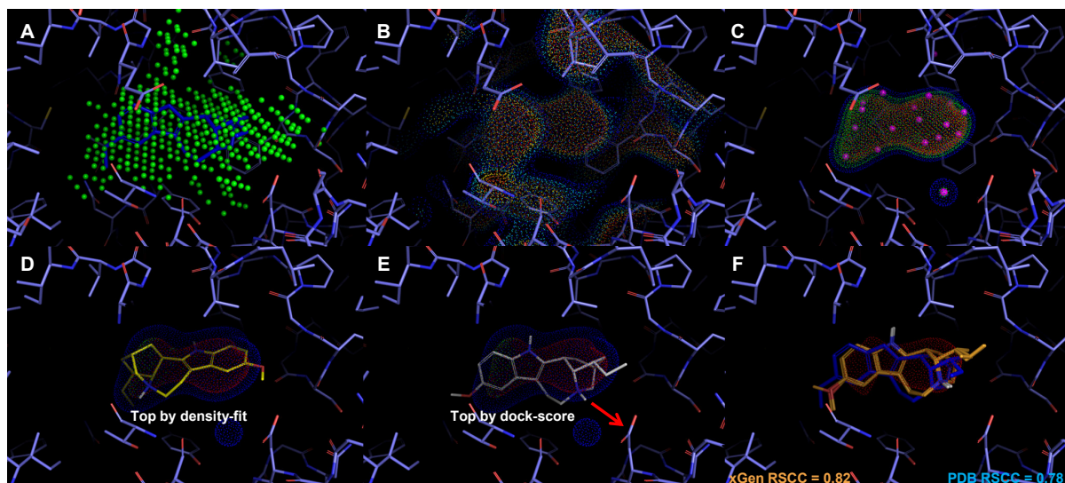
Figure 5.8 Fitting a ligand into a large volume of soft Cryo-EM density with no prior ligand placement (PDB 6DZZ): (A) Green spheres show the identified density blob; (B) Real-space experimental density contour points; (C) Spherical Gaussians (purple spheres) along with idealized density from de novo binding site identification; (D) Top-scoring density-fit pose into the de novo density approximation; (E) Top-scoring pose based on docking score optimization; (F) The final fully refined xGen ensemble.
