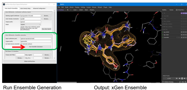
Figure 7.17 Step 4 of xGen ensemble generation: The final xGen ensemble.
