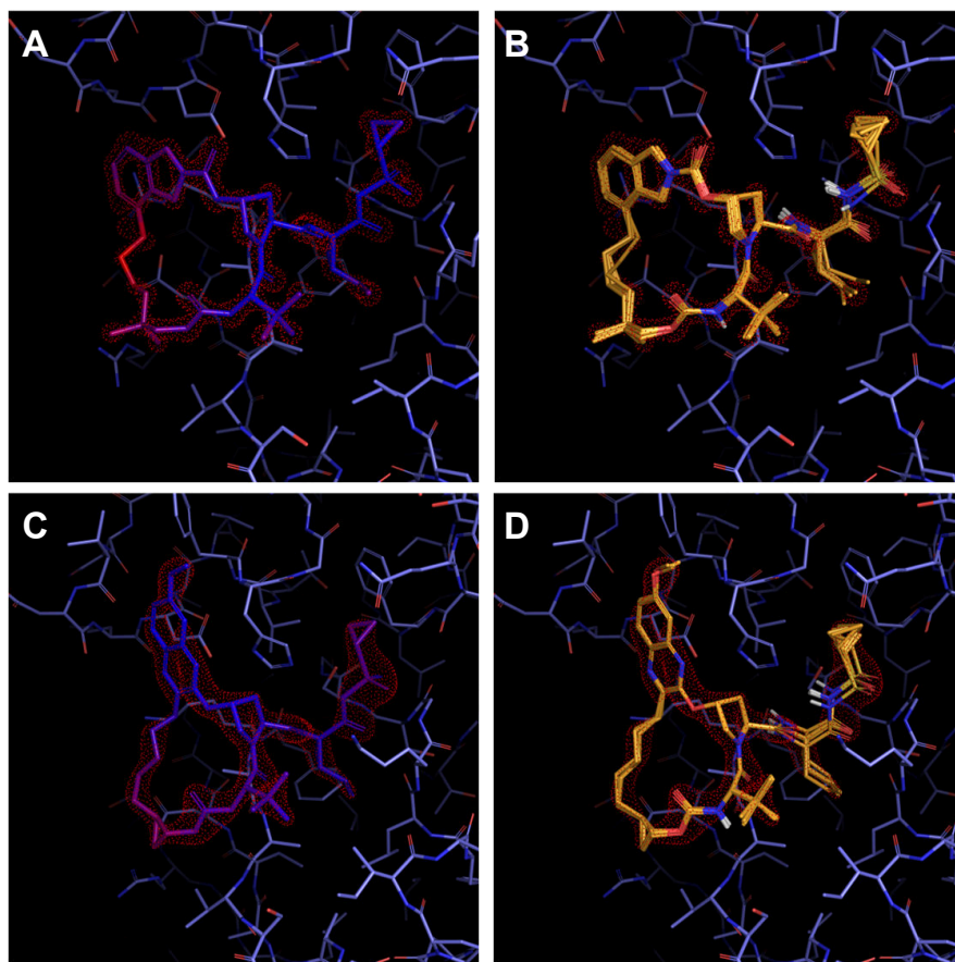
Figure 5.6 A: Deposited PDB ligand of 3SU3 with density contour. B: The xGen ensemble for the 3SU3 ligand. C: Deposited PDB ligand of 3SUE with density contour. D: The xGen ensemble for the 3SUE ligand.
