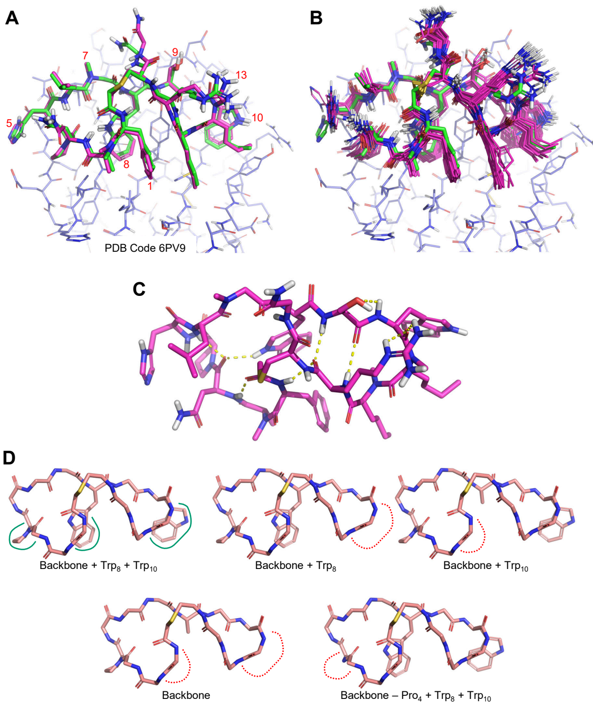
Figure 7.27 Solution ensemble for Pep-01 from NMR restrained conformational search: (A) the best-matching conformation from the ensemble (magenta carbons) and the bound state by crystallography (green carbons), with sidechains of specific residues numbered in red; (B) the 24 lowest energy non-redundant conformers (within 5 kcal/mol of the minimum, magenta) superimposed on the bound state (green), (C) the single lowest energy conformer (viewed from the solvent-exposed side) with H-bonds labeled; (D) five alternative molecular subfragments derived from the lowest energy conformer.
