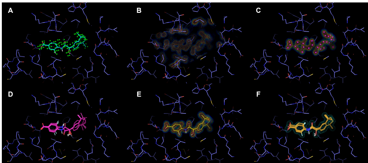
Figure 5.7 Fitting a ligand into a volume of density with no prior ligand placement (PDB: 1EXX): (A) Green spheres show the automatically detected density site blob (PDB ligand shown for reference only); (B) Experimental density contours; (C) Idealized density with spherical Gaussian centers shown as spheres; (D) All conformers from the initial rough fit into the de novo density approximation; (E) Top conformer of the approximate ensemble from which the final density approximation is built and ligand conformers are produced for the final ensemble; (F) The final xGen ensemble.
