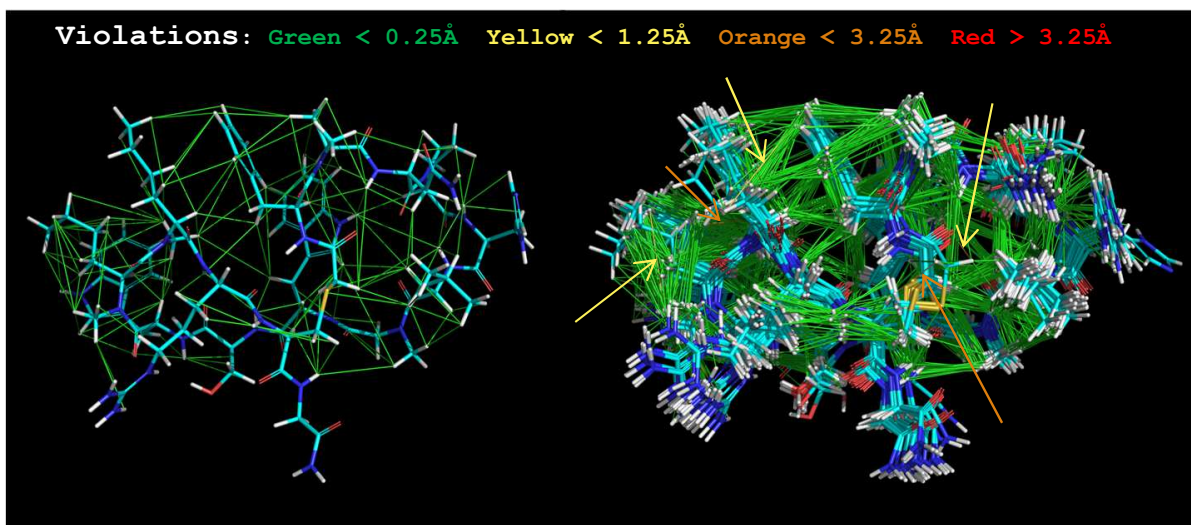
Figure 7.25 Display of NMR distance violations: green lines are satisfied distance restraints, yellow are minor violations, orange are significant, and red are large.
