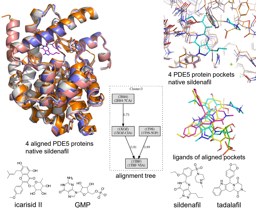
Figure 3.10 Four aligned PDE5 structures are shown in ribbons and in sticks with native sildenafil in the pocket of both depictions. The alignment of the structures (bound to icarisid II, GMP, sildenafil, and tadalafil) shows the movement possible within the pocket (upper right). The alignment tree of four PDE5 structures shows the degrees of similarity between the aligned protein binding sites.
