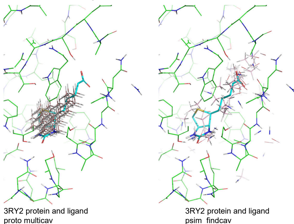
Figure 3.5 Shown are the crystallographic 3RY2 protein (green) and instantiation 1 of 4 for biotin (cyan). The thin sticks show the sites marked by two automatic cavity finding protocols: left in tan sticks, biotin site 1 found by multicav, and right in pink sticks, the protomol from psim_findcav.
