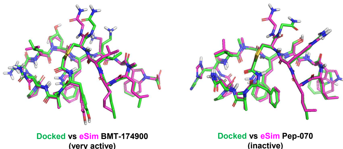
Figure 7.29 Comparison of predicted bound poses of two MCPs using SF-Dock (green) and eSim (magenta).
